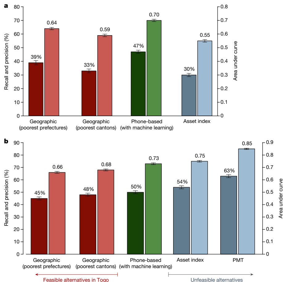
Fig. 1 | Comparing Novissi targeting to alternatives. a, b , The performance of phone-based targeting (green) compared with alternative approaches that were feasible (red) and unfeasible (blue) in Togo in 2020. Targeting is evaluated for the actual rural Novissi programme ( a ), which focused on Togo's 100 poorest cantons (using a 2020 survey representative of mobile subscribers in the 100 cantons, where PMT is a ground truth for poverty since consumption data was not collected in the phone survey); and a hypothetical nationwide
